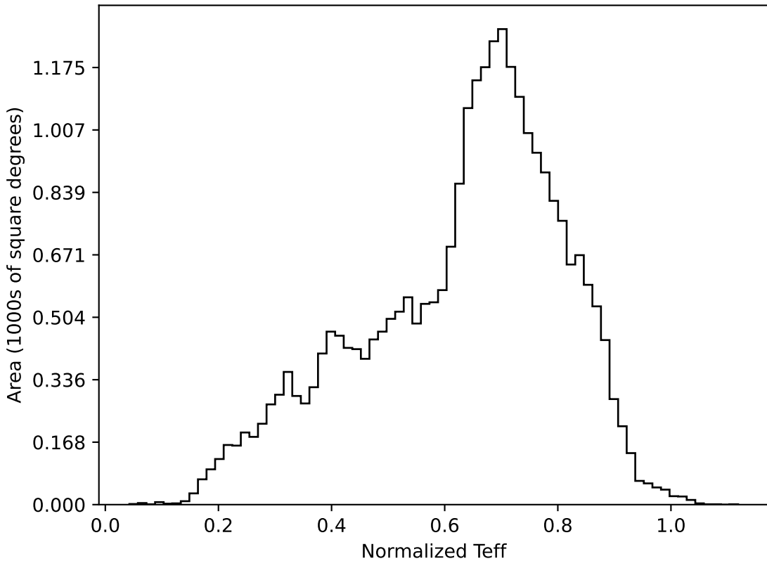
weather_cloudso31v3.4_10yrs All sky all bands: Normalized Teff
