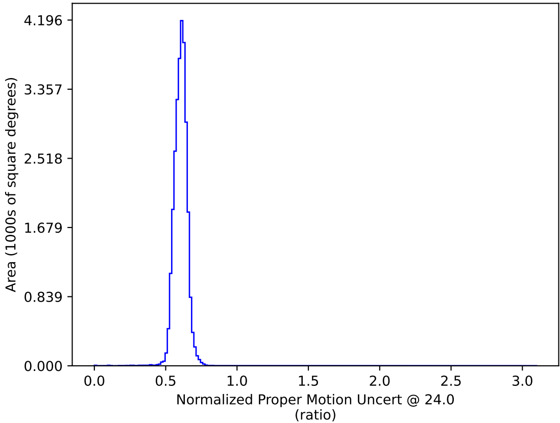
weather_cloudso31v3.4_10yrs All sky: Normalized Proper Motion Uncert @ 24.0
