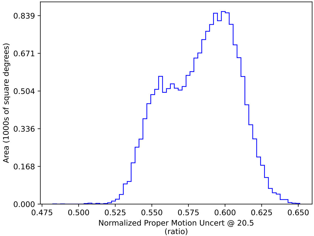
weather_cloudso31v3.4_10yrs WFD: Normalized Proper Motion Uncert @ 20.5
