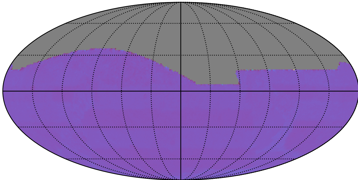
weather_cloudso31v3.4_10yrs All sky: Normalized Proper Motion Uncert @ 20.5
