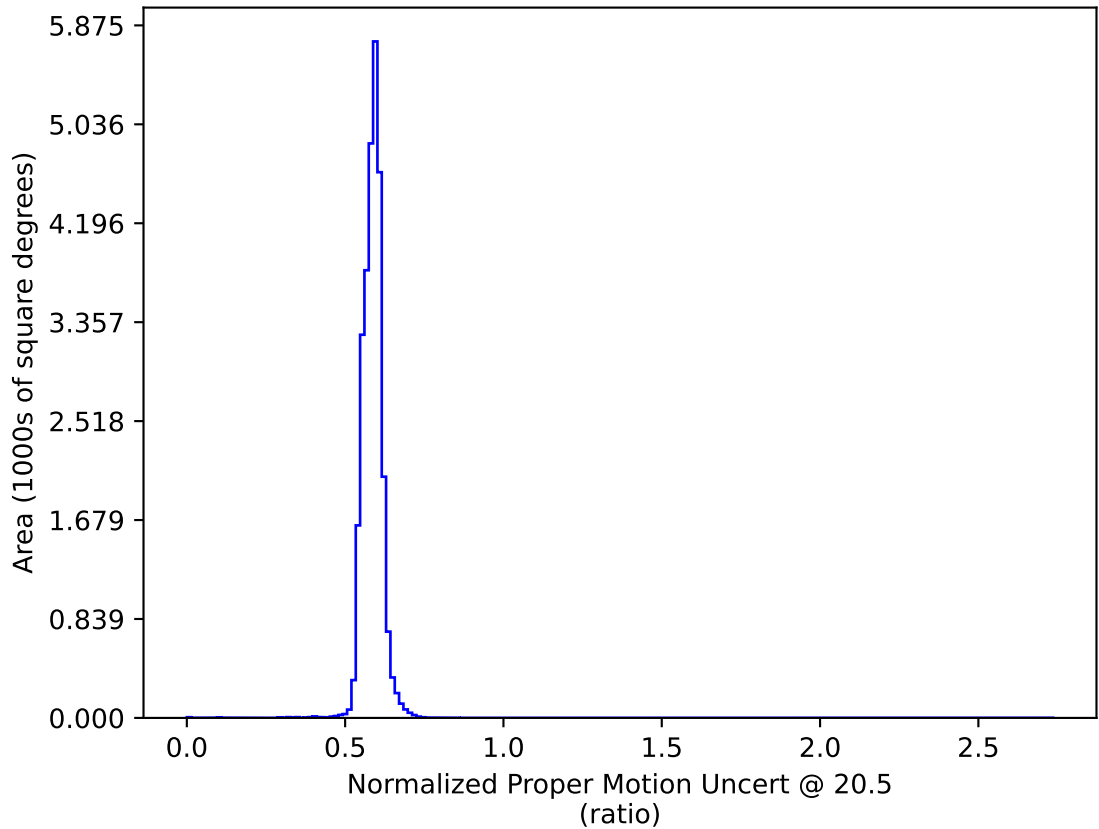
weather_cloudso31v3.4_10yrs All sky: Normalized Proper Motion Uncert @ 20.5
