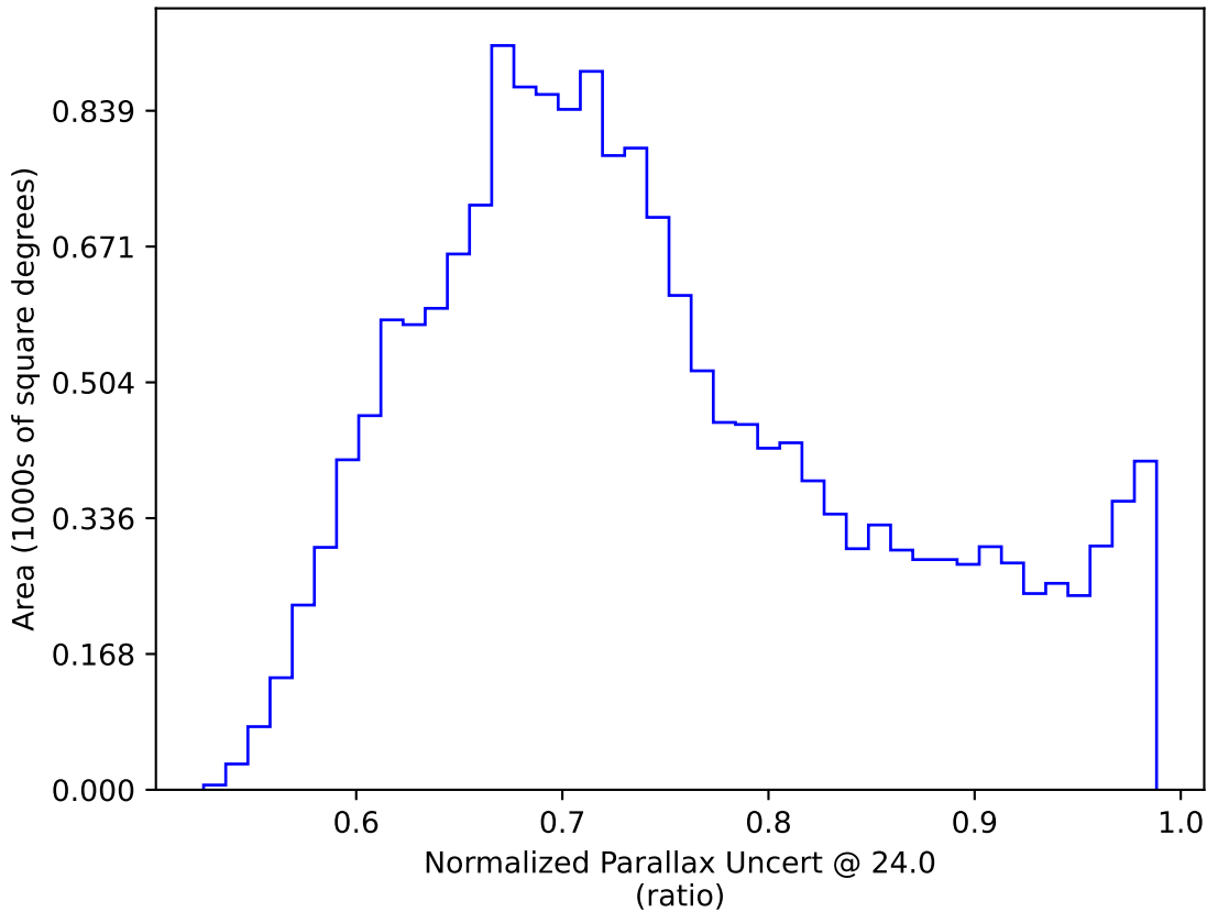
weather_cloudso31v3.4_10yrs WFD: Normalized Parallax Uncert @ 24.0
