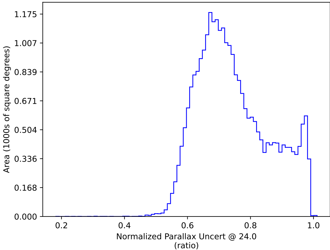
weather_cloudso31v3.4_10yrs All sky: Normalized Parallax Uncert @ 24.0
