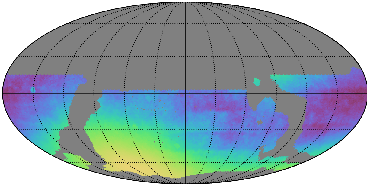
weather_cloudso31v3.4_10yrs WFD: Normalized Parallax Uncert @ 22.4
