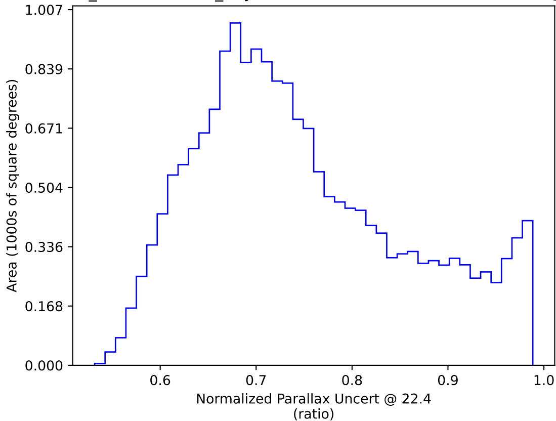
weather_cloudso31v3.4_10yrs WFD: Normalized Parallax Uncert @ 22.4
