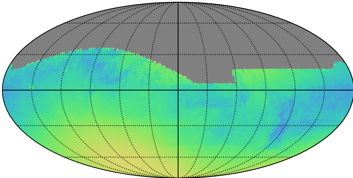
weather_cloudso31v3.4_10yrs All sky: Normalized Parallax Uncert @ 22.4
