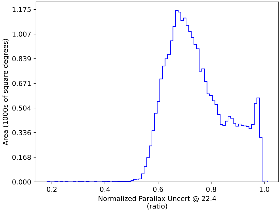
weather_cloudso31v3.4_10yrs All sky: Normalized Parallax Uncert @ 22.4
