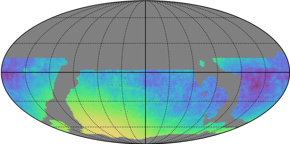
weather_cloudso31v3.4_10yrs WFD y band only: Normalized Parallax Uncert @ 21.3
