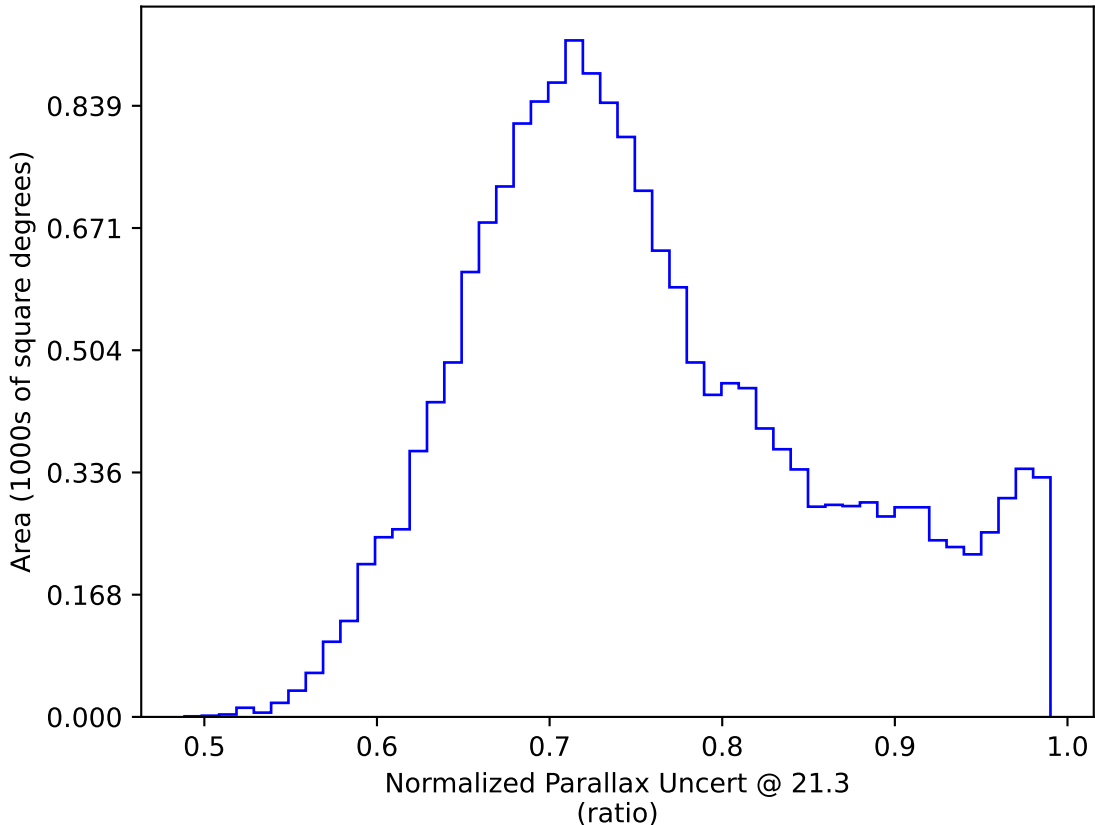
weather_cloudso31v3.4_10yrs WFD y band only: Normalized Parallax Uncert @ 21.3
