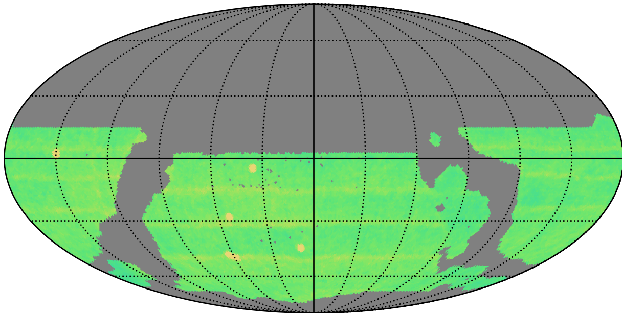
weather_cloudso31v3.4_10yrs WFD all bands: N Unique Nights
