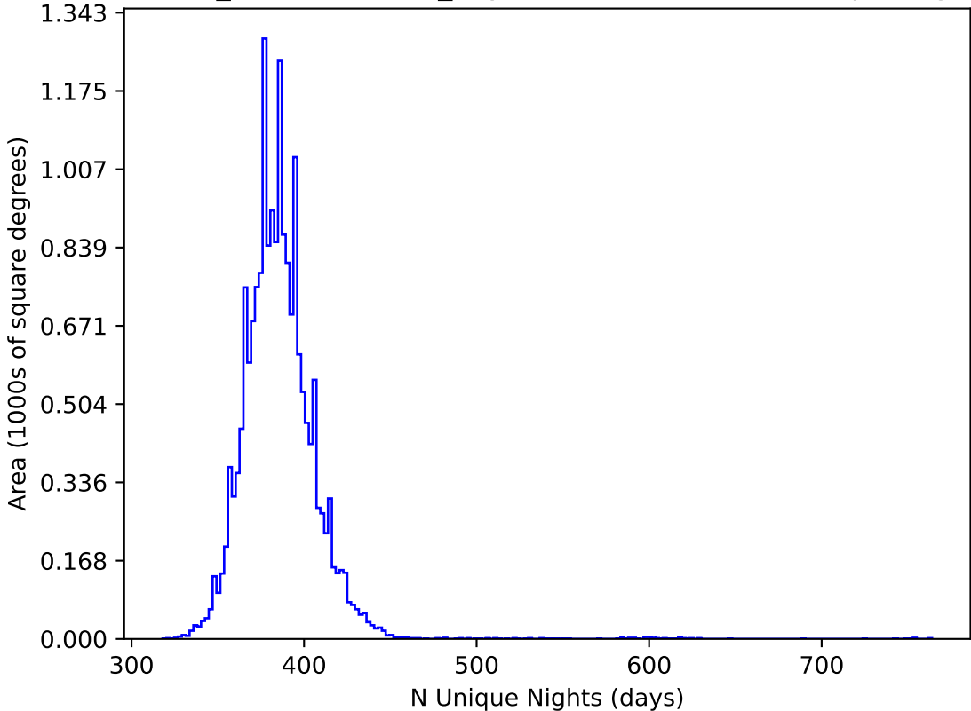
weather_cloudso31v3.4_10yrs WFD all bands: N Unique Nights
