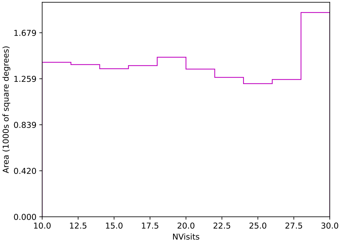
weather_cloudso31v3.4_10yrs Yr 3-4 z band: NVisits
