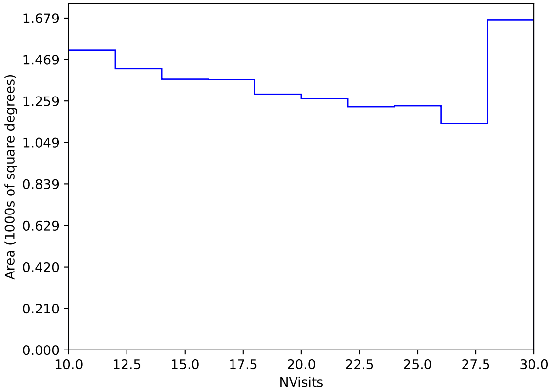
weather_cloudso31v3.4_10yrs Yr 3-4 y band: NVisits
