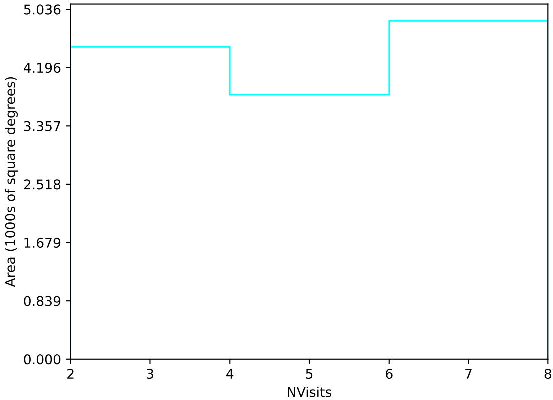
weather_cloudso31v3.4_10yrs Yr 3-4 u band: NVisits
