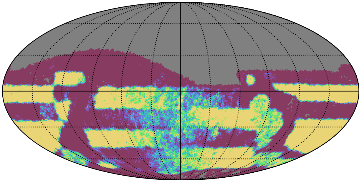
weather_cloudso31v3.4_10yrs Yr 3-4 r band: NVisits
