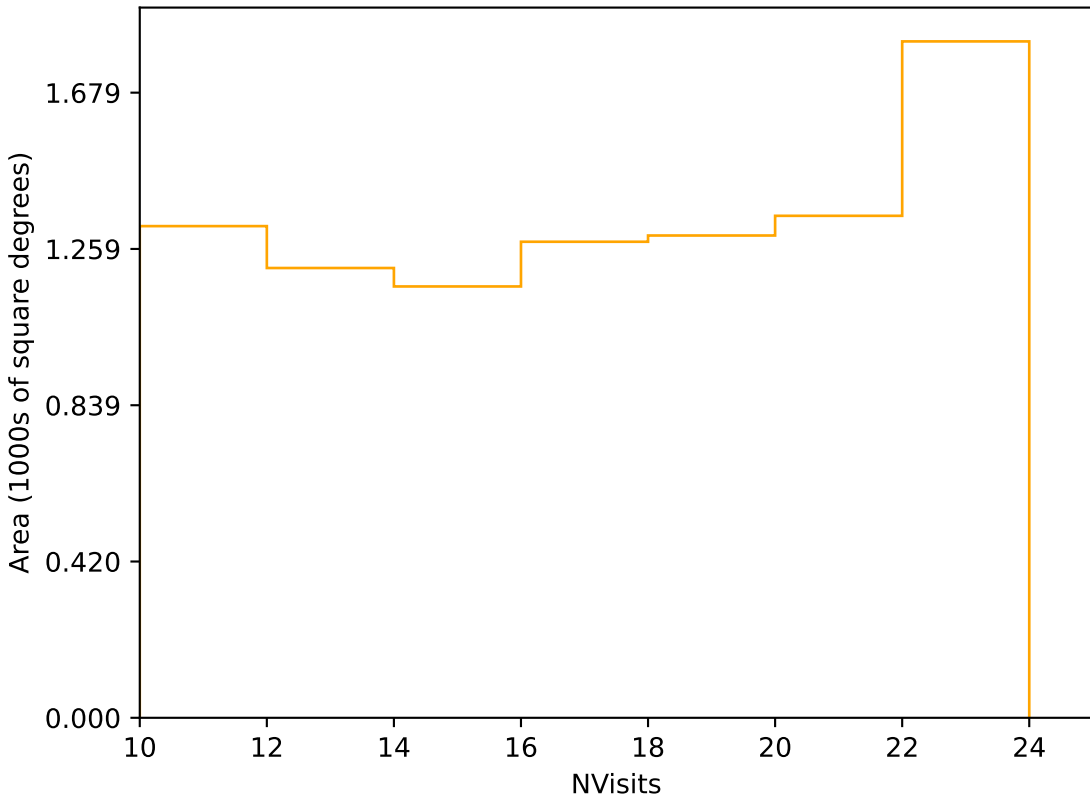
weather_cloudso31v3.4_10yrs Yr 3-4 r band: NVisits
