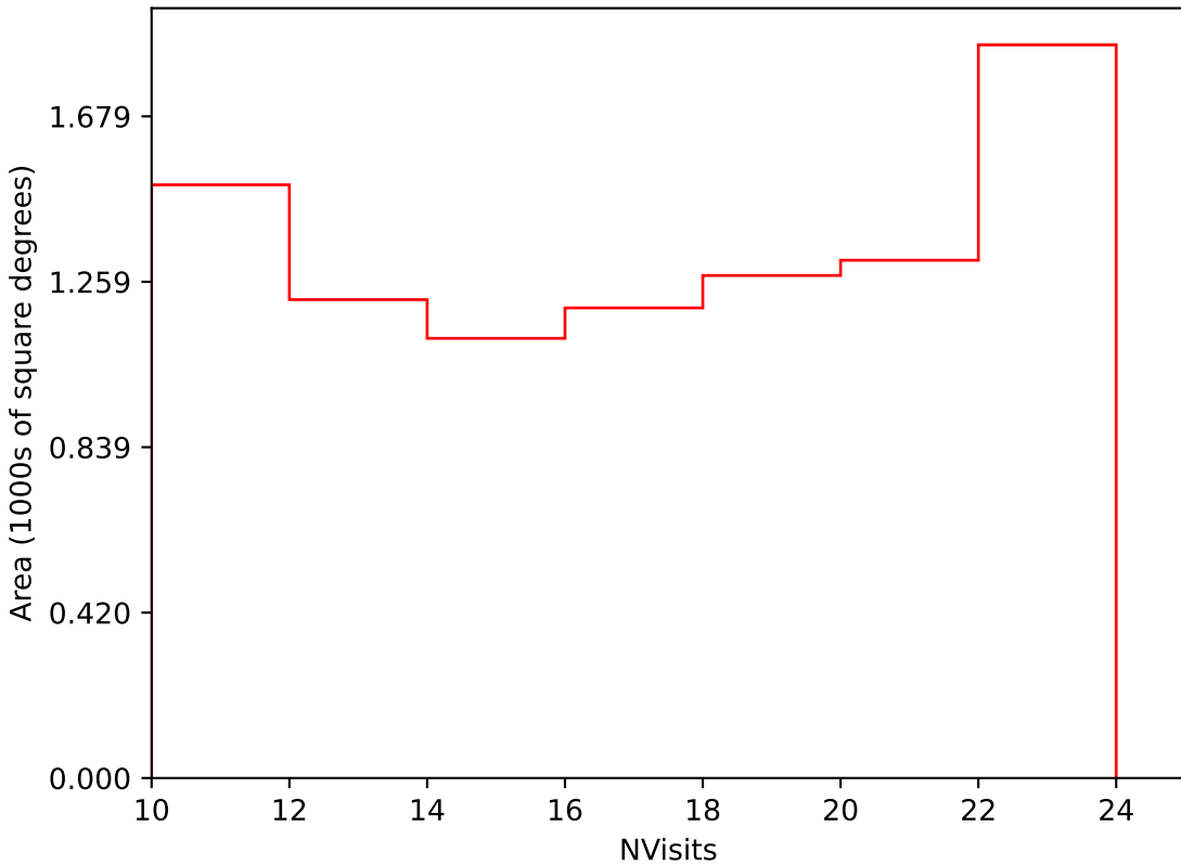
weather_cloudso31v3.4_10yrs Yr 3-4 i band: NVisits
