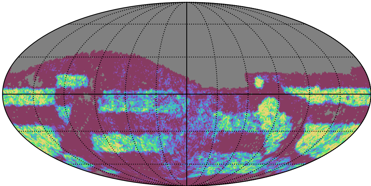
weather_cloudso31v3.4_10yrs Yr 3-4 g band: NVisits
