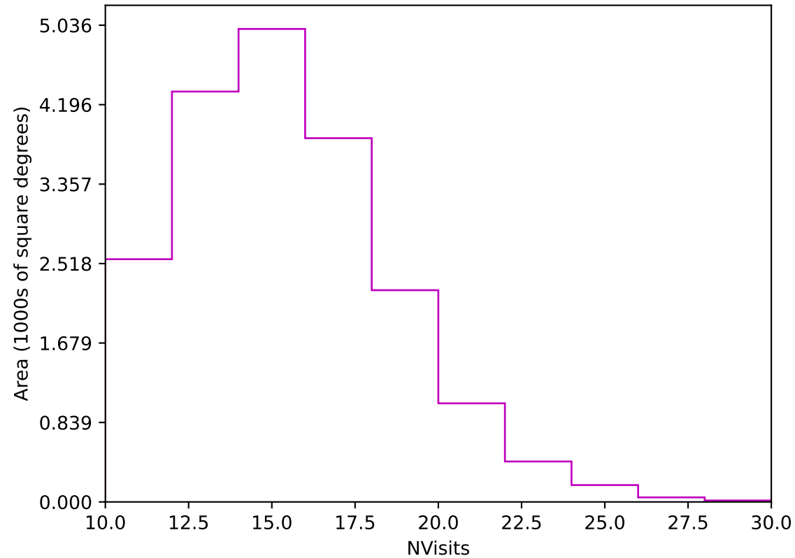
weather_cloudso31v3.4_10yrs Yr 1 z band: NVisits
