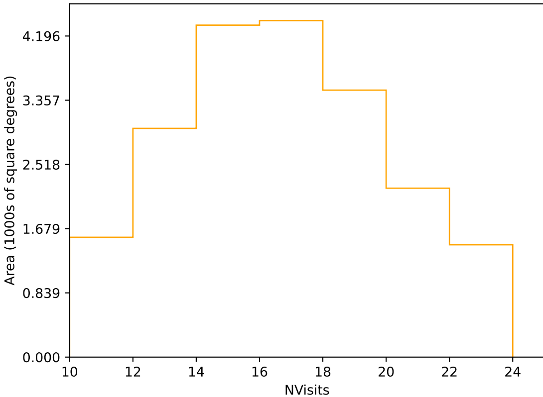
weather_cloudso31v3.4_10yrs Yr 1 r band: NVisits
