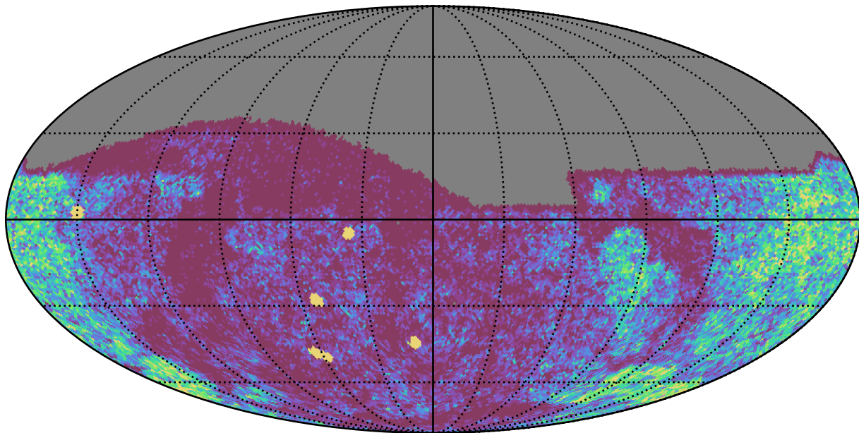
weather_cloudso31v3.4_10yrs Yr 1 g band: NVisits
