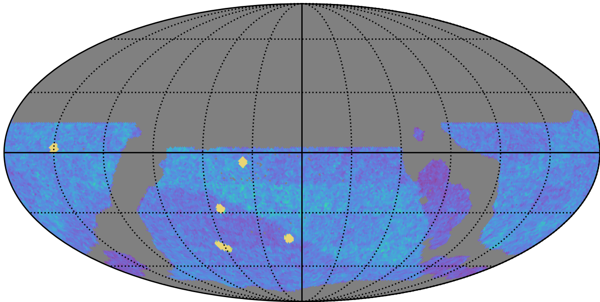
weather_cloudso31v3.4_10yrs WFD z band: NVisits
