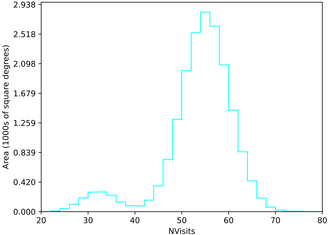
weather_cloudso31v3.4_10yrs WFD u band: NVisits
