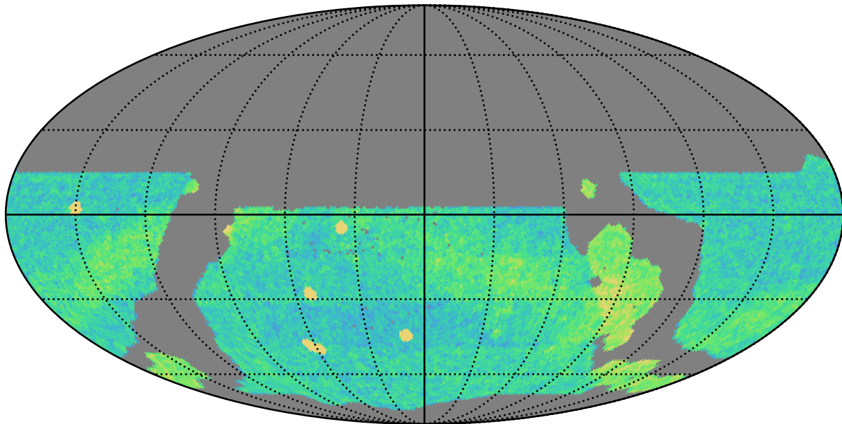
weather_cloudso31v3.4_10yrs WFD r band: NVisits
