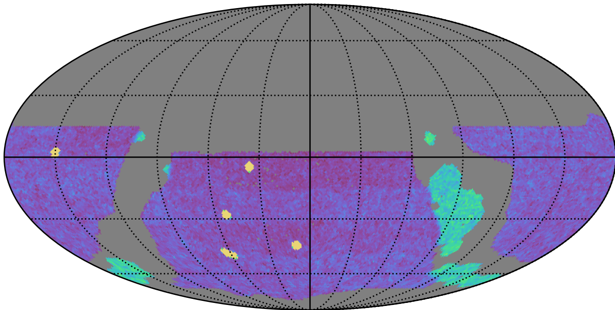
weather_cloudso31v3.4_10yrs WFD g band: NVisits
