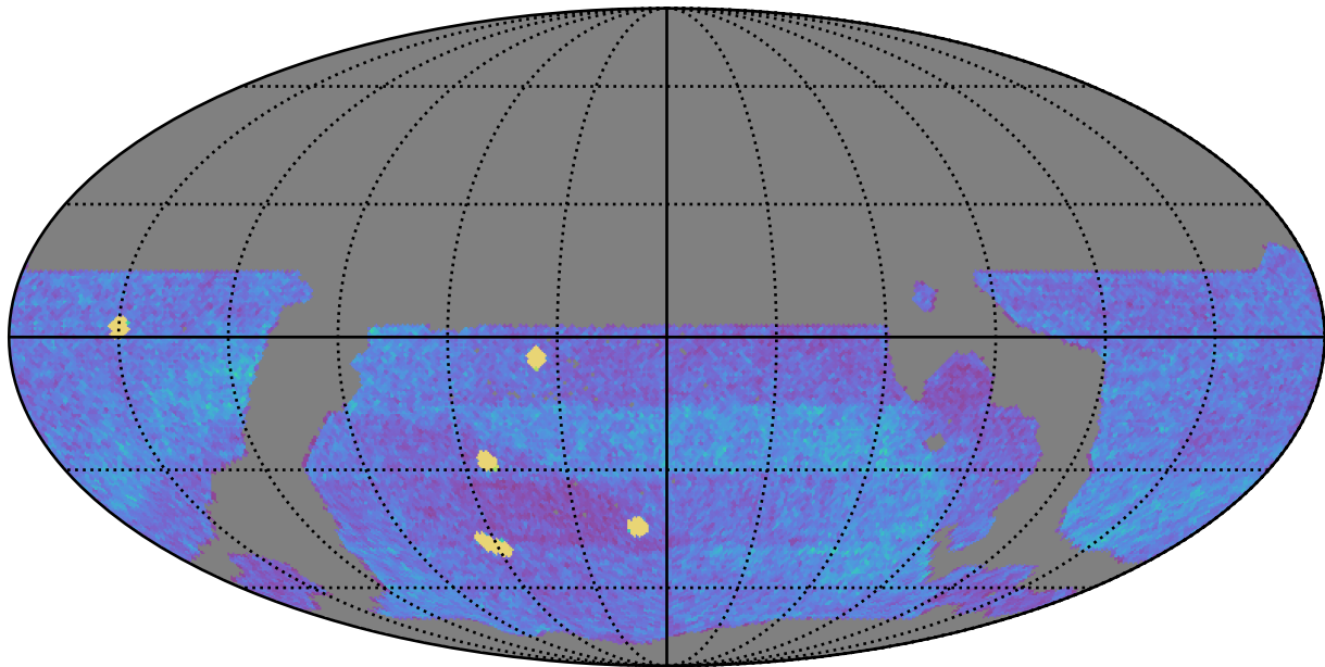
weather_cloudso31v3.4_10yrs WFD all bands: NVisits
