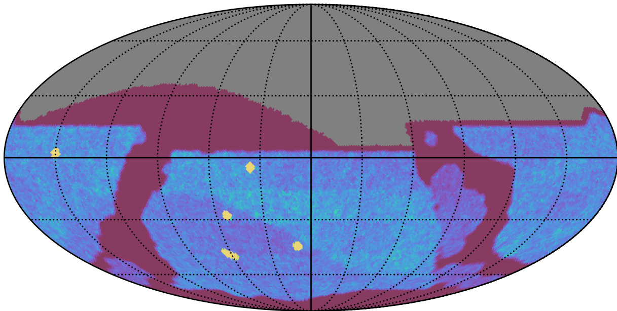
weather_cloudso31v3.4_10yrs All sky z band: NVisits
