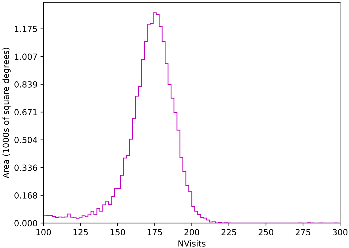
weather_cloudso31v3.4_10yrs All sky z band: NVisits
