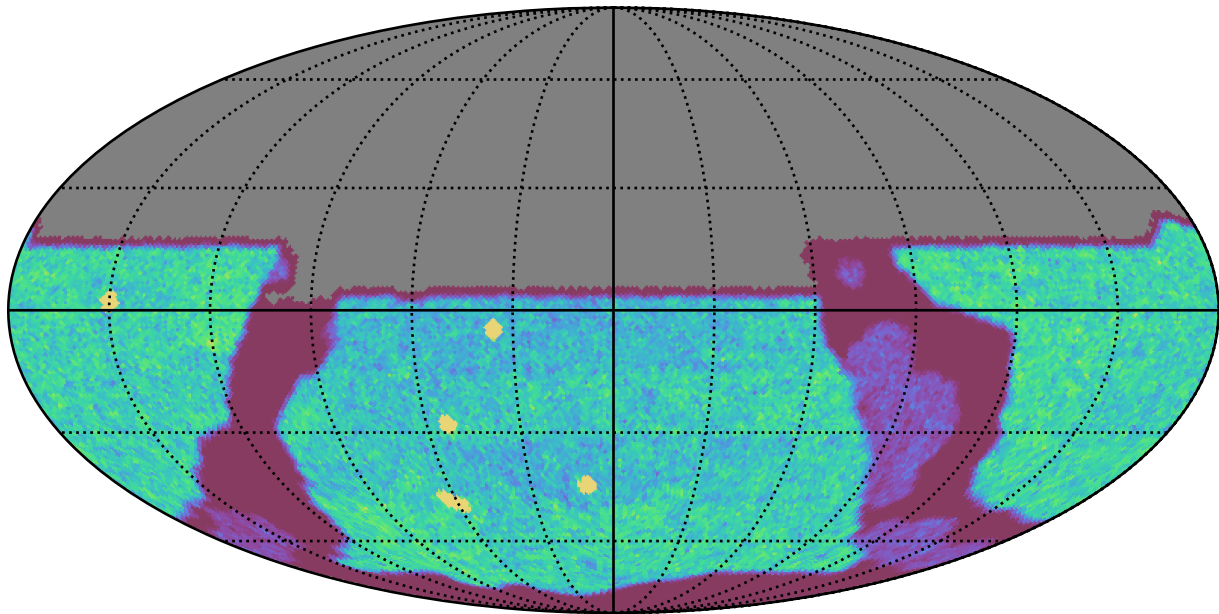
weather_cloudso31v3.4_10yrs All sky u band: NVisits
