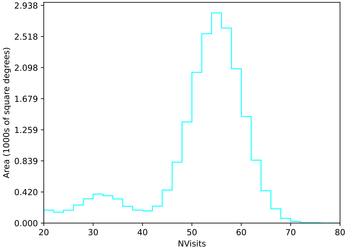
weather_cloudso31v3.4_10yrs All sky u band: NVisits
