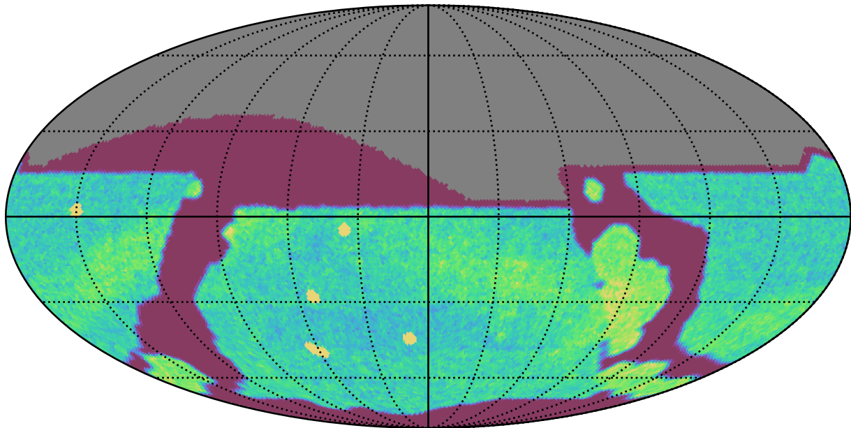
weather_cloudso31v3.4_10yrs All sky r band: NVisits
