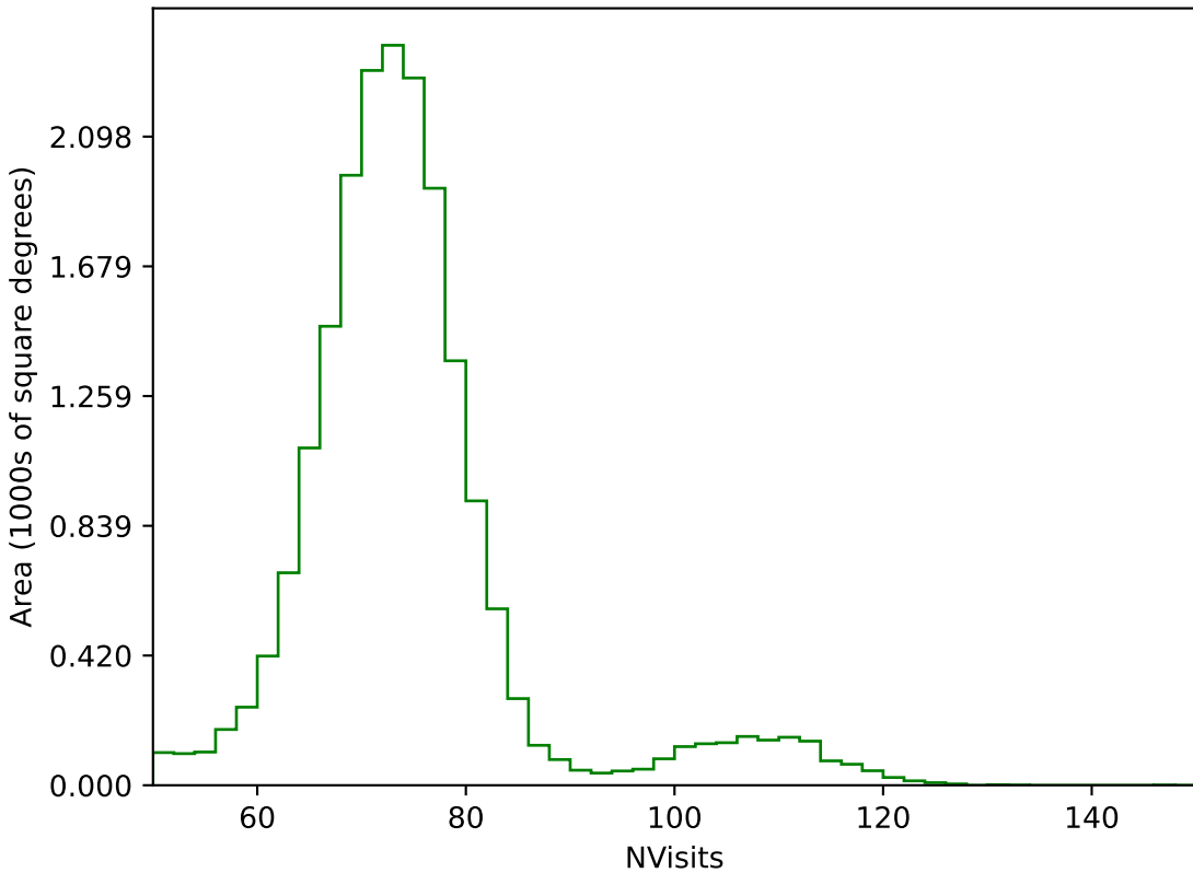
weather_cloudso31v3.4_10yrs All sky g band: NVisits
