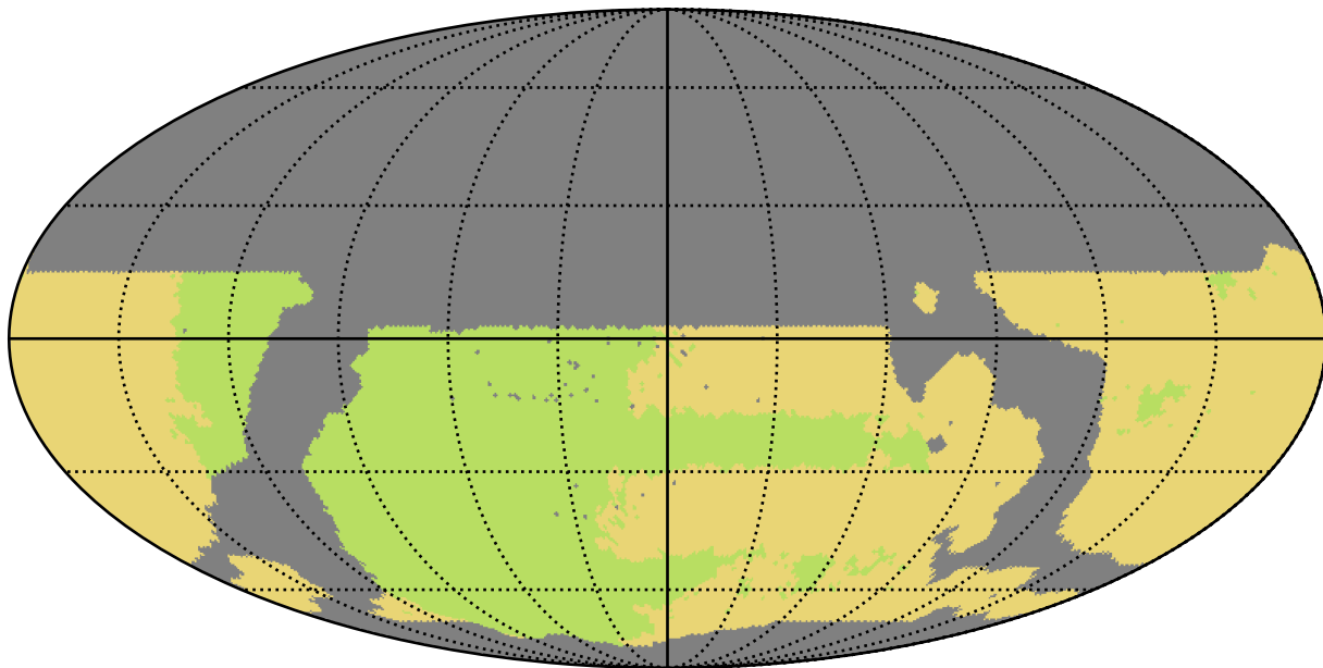
weather_cloudso31v3.4_10yrs WFD all bands: NSeasons
