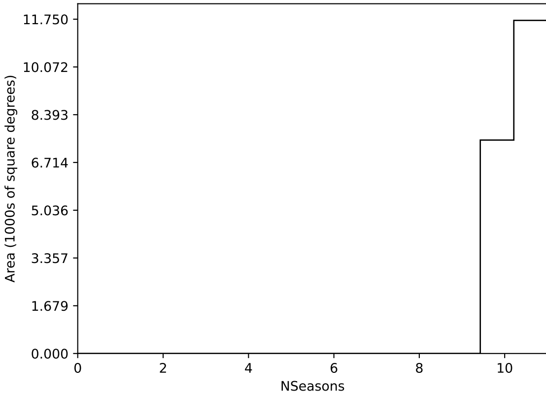
weather_cloudso31v3.4_10yrs WFD all bands: NSeasons
