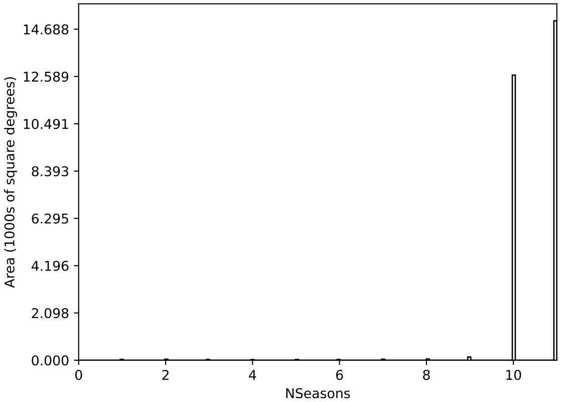
weather_cloudso31v3.4_10yrs All sky all bands: NSeasons
