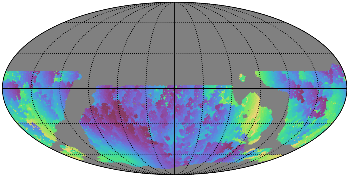
weather_cloudso31v3.4_10yrs WFD u band: Min solarElong
