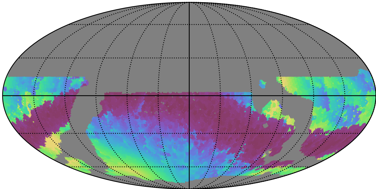
weather_cloudso31v3.4_10yrs WFD r band: Min solarElong
