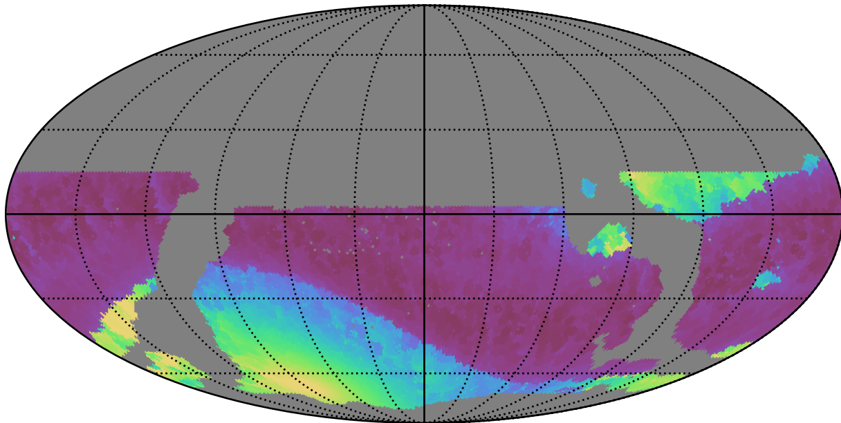
weather_cloudso31v3.4_10yrs WFD all bands: Min solarElong
