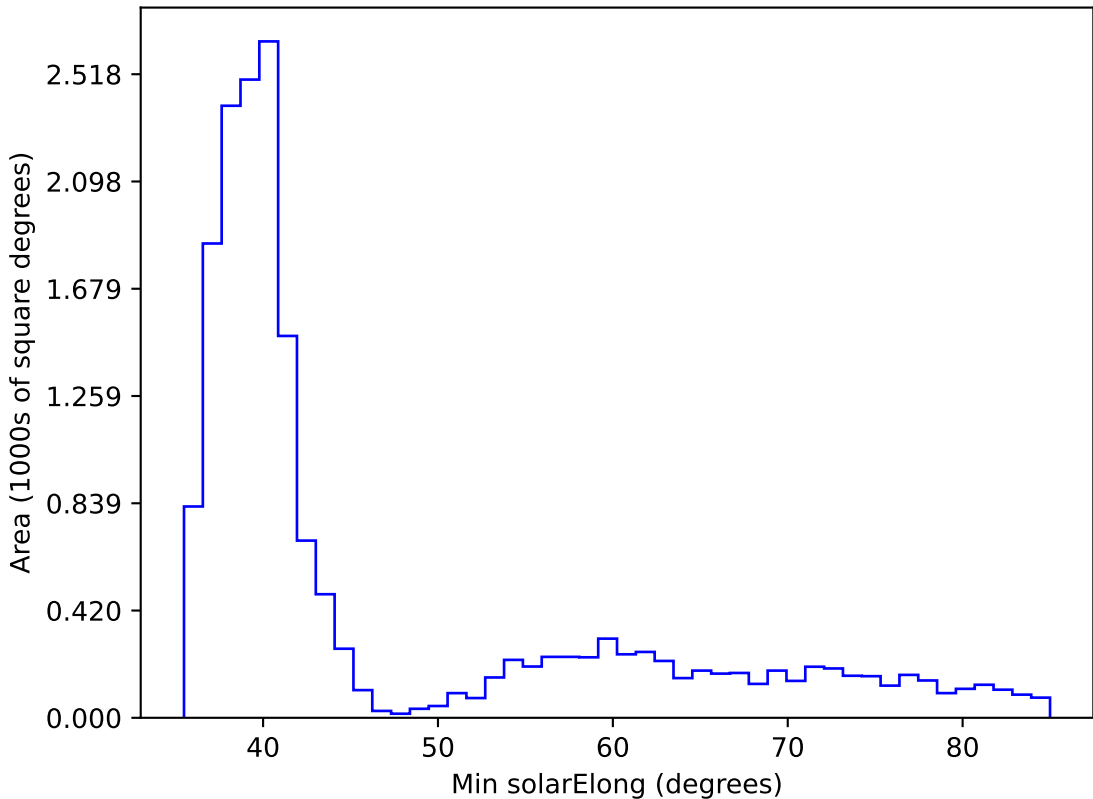
weather_cloudso31v3.4_10yrs WFD all bands: Min solarElong
