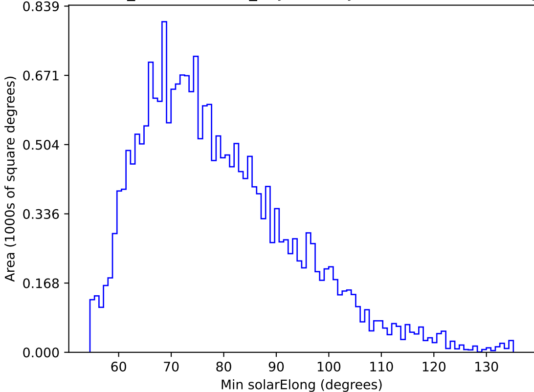
weather_cloudso31v3.4_10yrs All sky u band: Min solarElong
