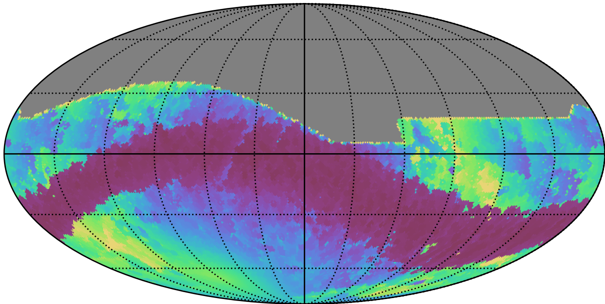
weather_cloudso31v3.4_10yrs All sky r band: Min solarElong
