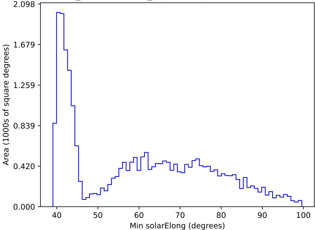
weather_cloudso31v3.4_10yrs All sky r band: Min solarElong
