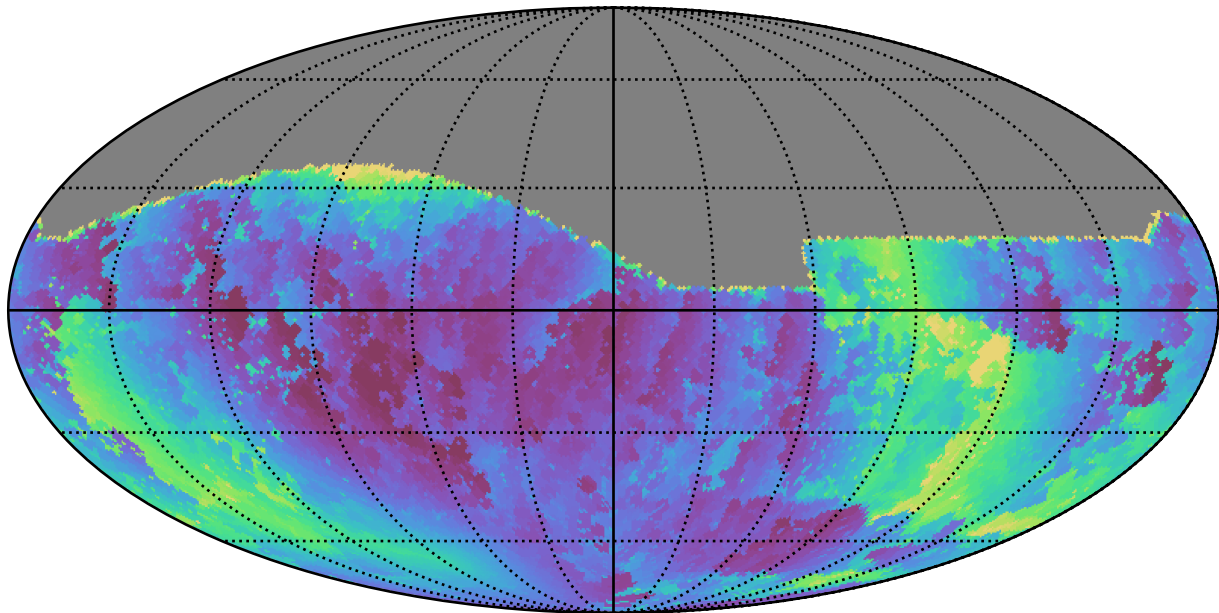
weather_cloudso31v3.4_10yrs All sky g band: Min solarElong
