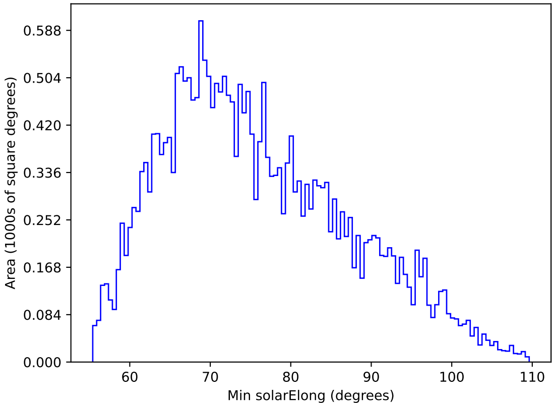
weather_cloudso31v3.4_10yrs All sky g band: Min solarElong
