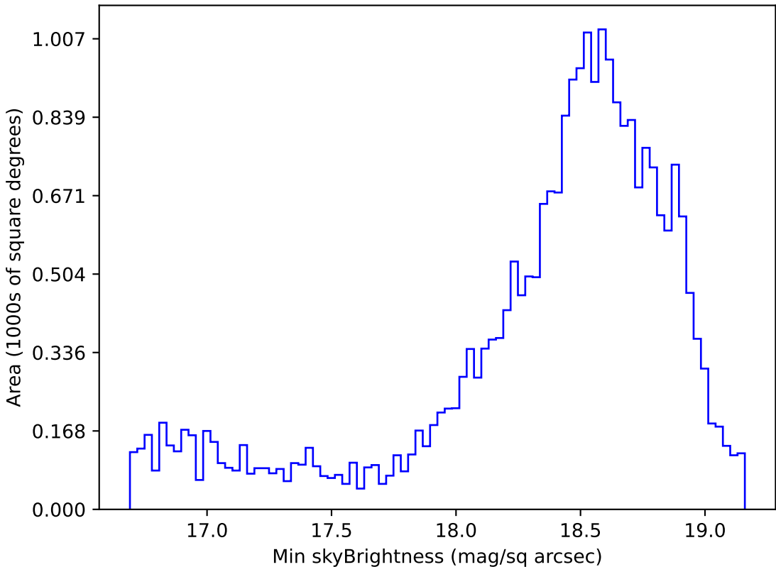
weather_cloudso31v3.4_10yrs Yr 1 z band: Min skyBrightness
