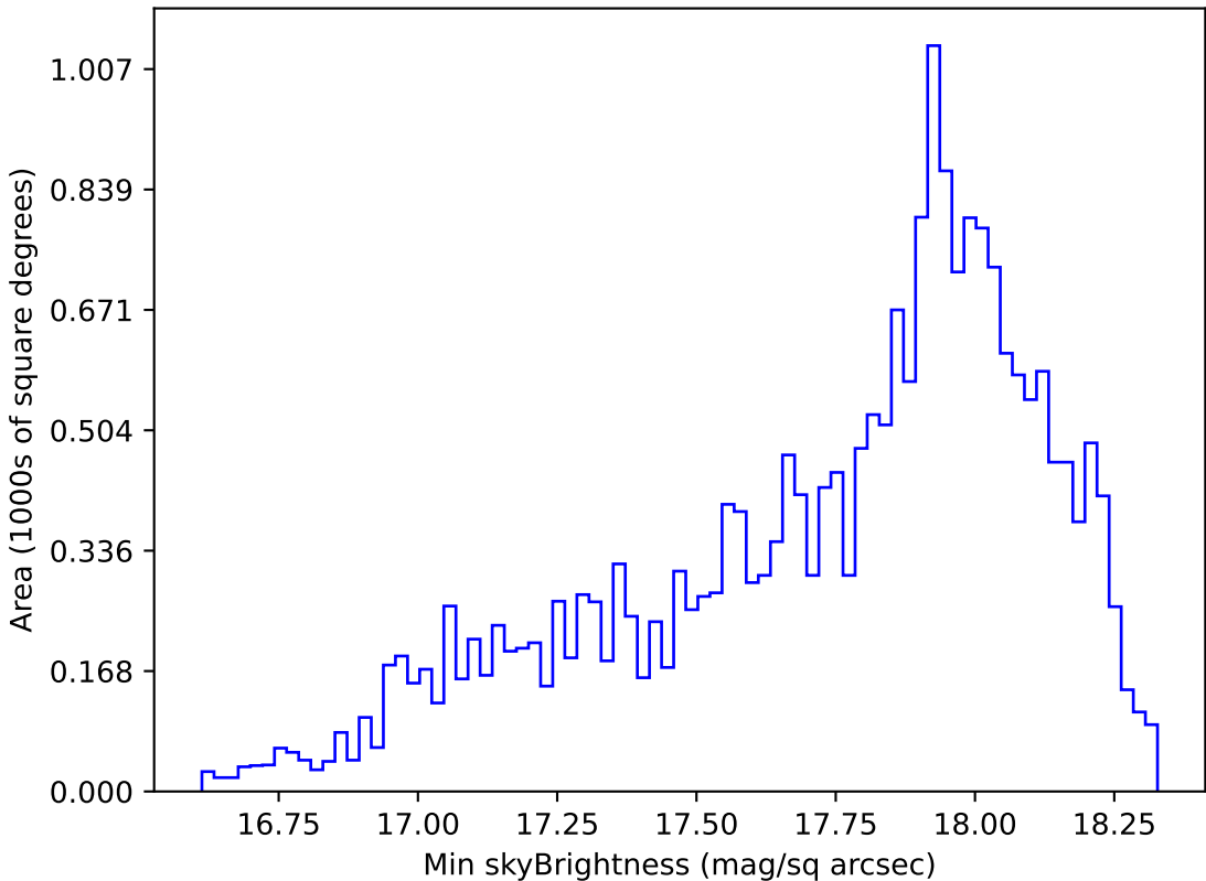
weather_cloudso31v3.4_10yrs Yr 1 y band: Min skyBrightness
